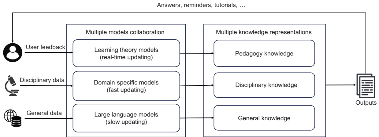
Fig. 1 Large language model and domain-specific model collaboration (LDMC) framework
